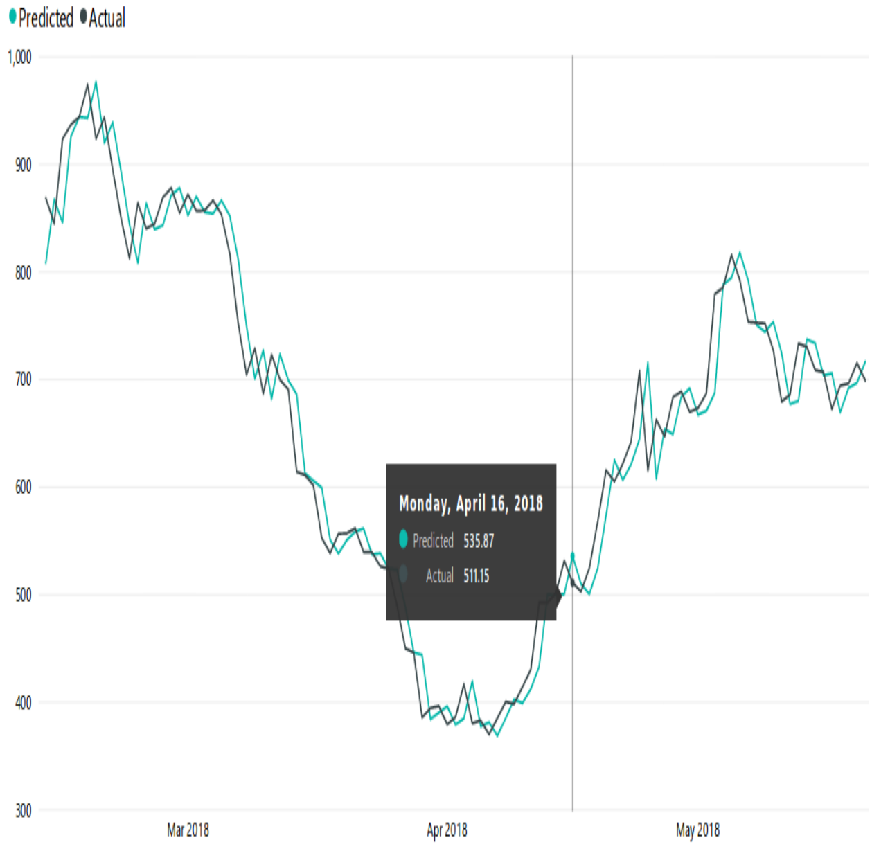
Figure 3.11 Screenshot for Actual vs. Predicted price of Ether
