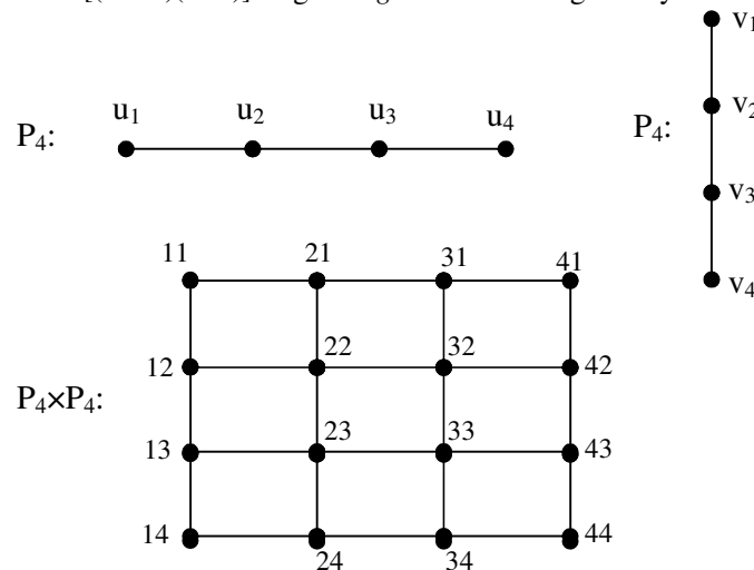
Figure 1. Grid P_4 \times P_4
