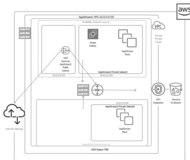
Fig. 1. Architecture Model of AppStream
