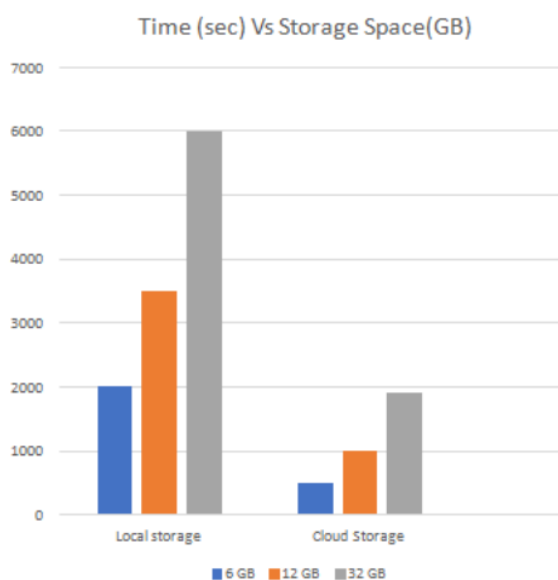
Fig. 5. Time vs Storage Space
